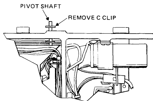
FIGURE 7 CARTRIDGE GUIDE REMOVAL
