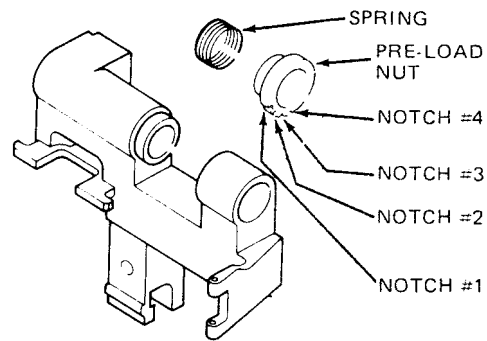
FIGURE 8 CARRIAGE ASSEMBLY
